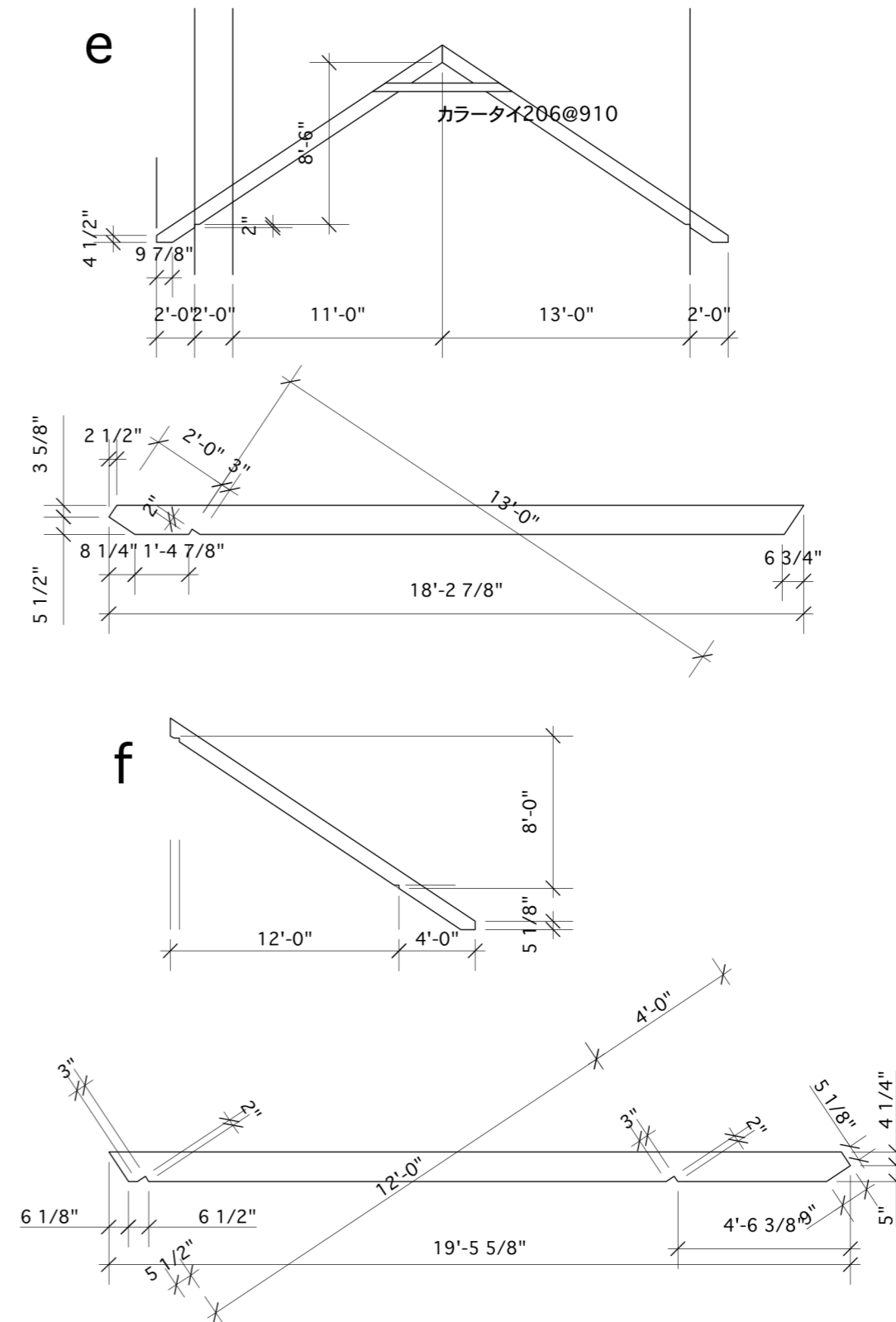
垂木姿図 縮尺 1/50
